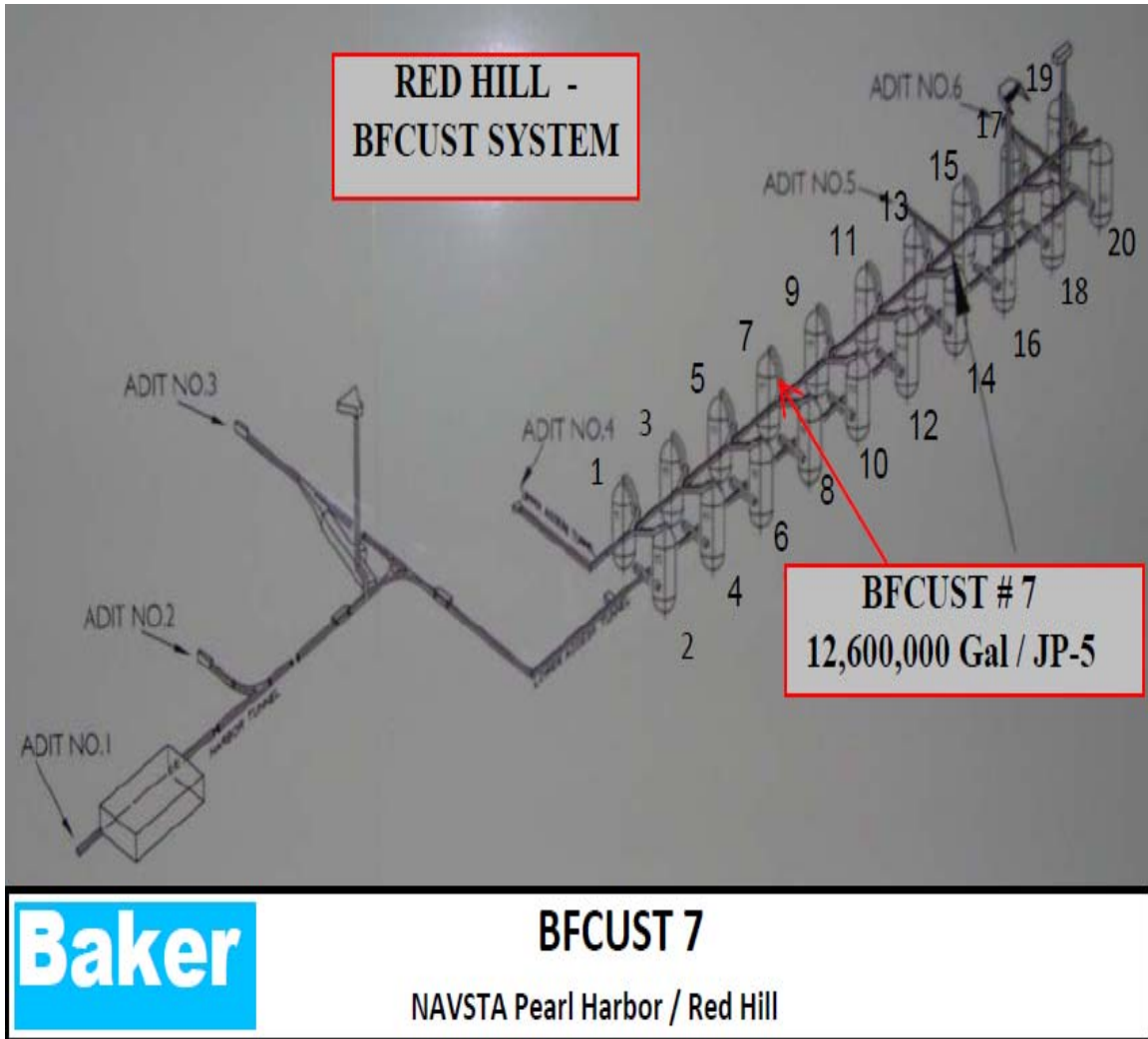
Figure 1-1: RED HILL – System Layout
