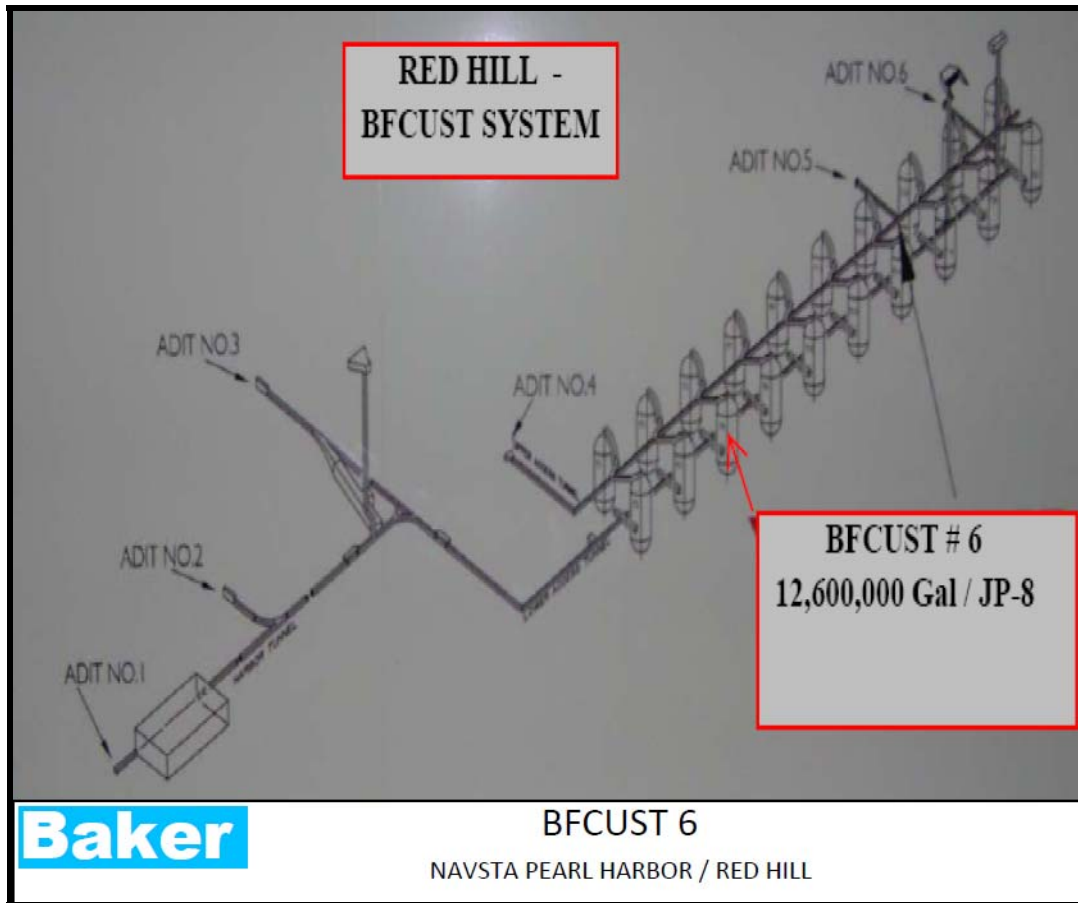
Figure 1-1: RED HILL – System Layout
