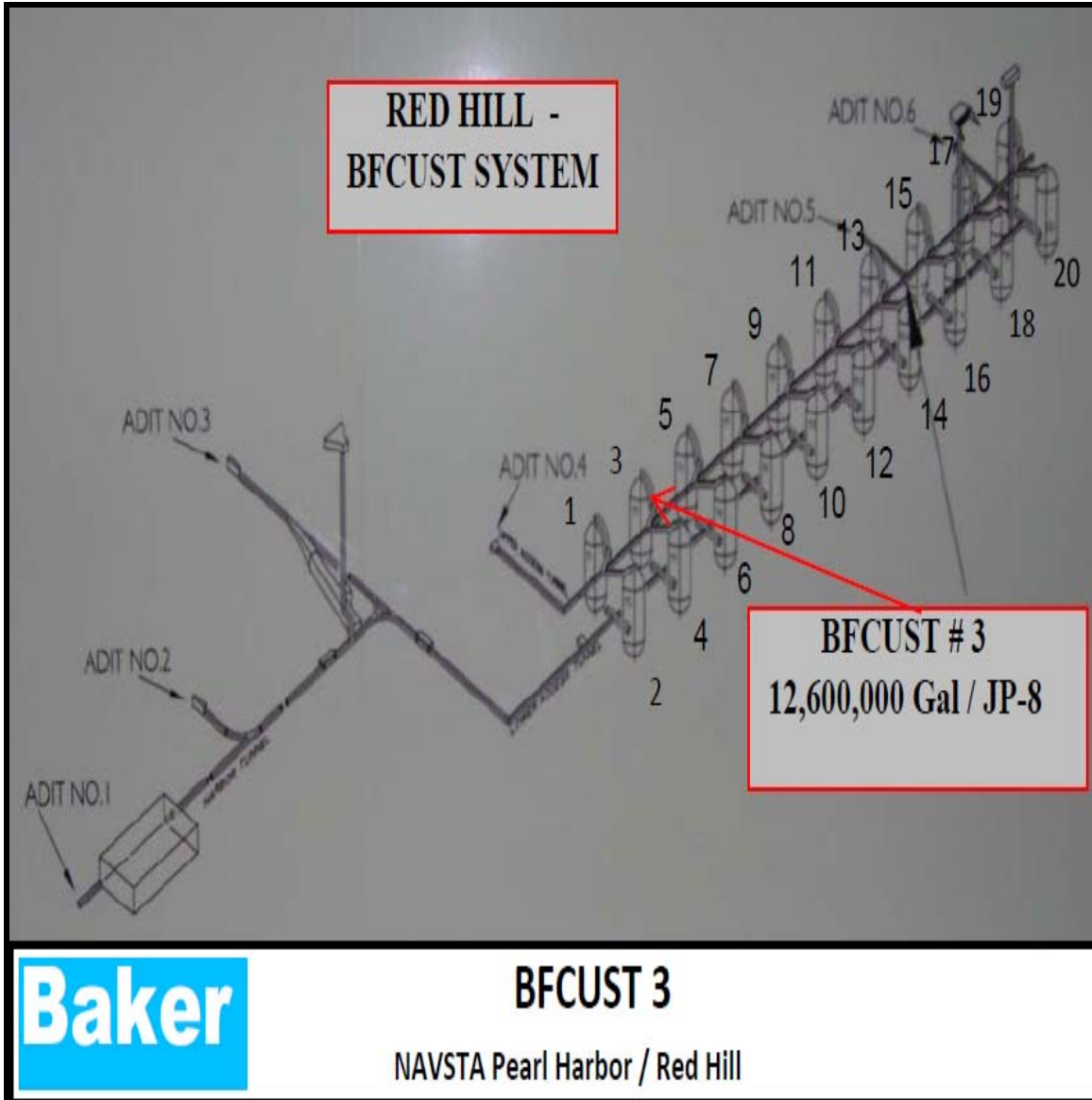
Figure 1-1: RED HILL – System Layout
