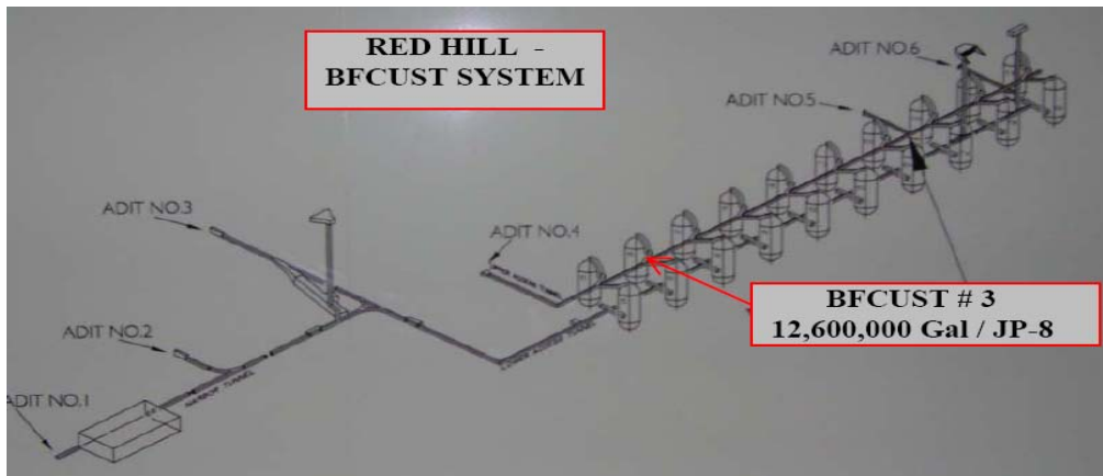
Figure 1: RED HILL – BFCUST SYSTEM – BFCUST # 3
