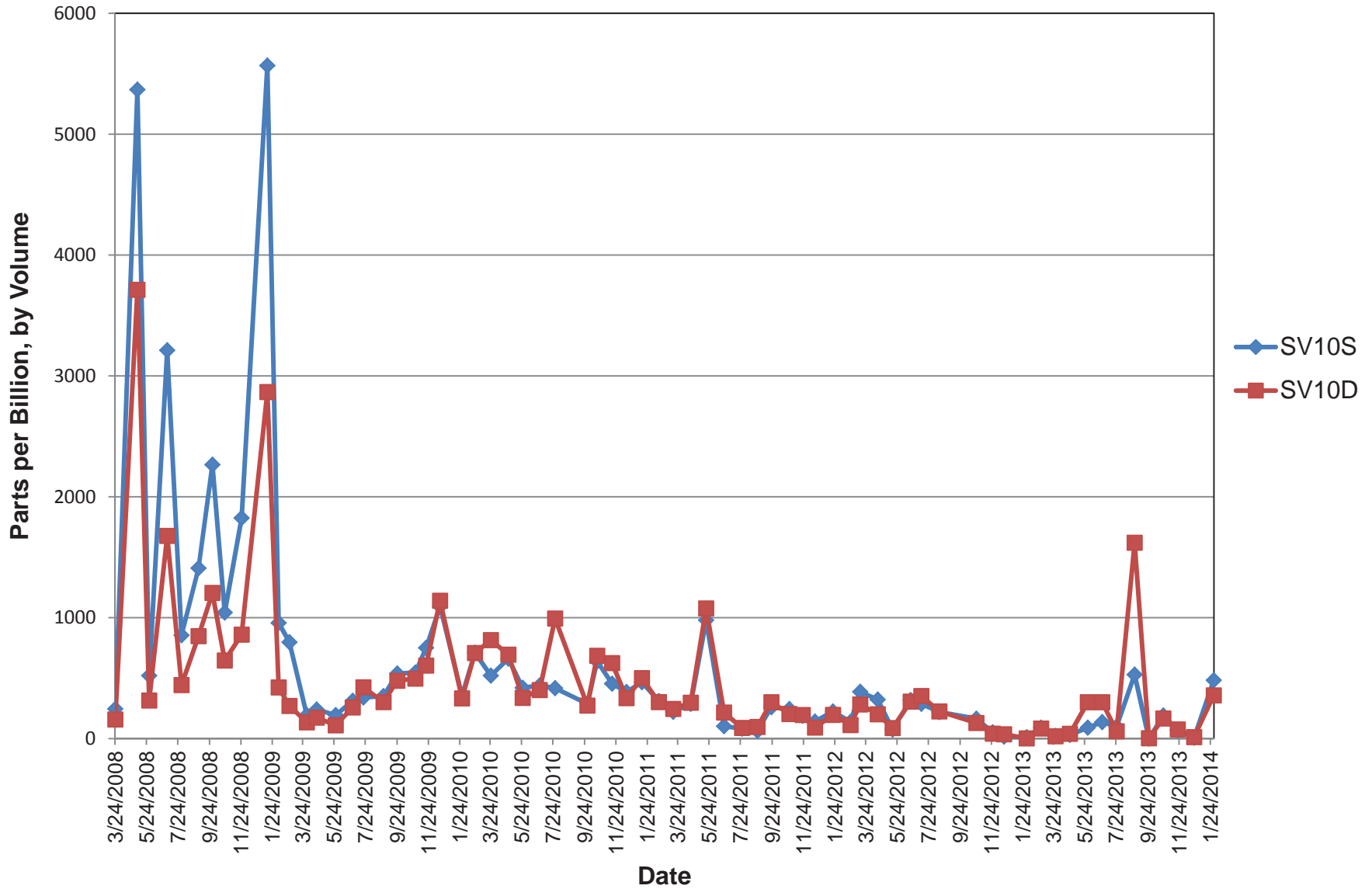
Figure 9 Soil Vapor Measurements SV10
