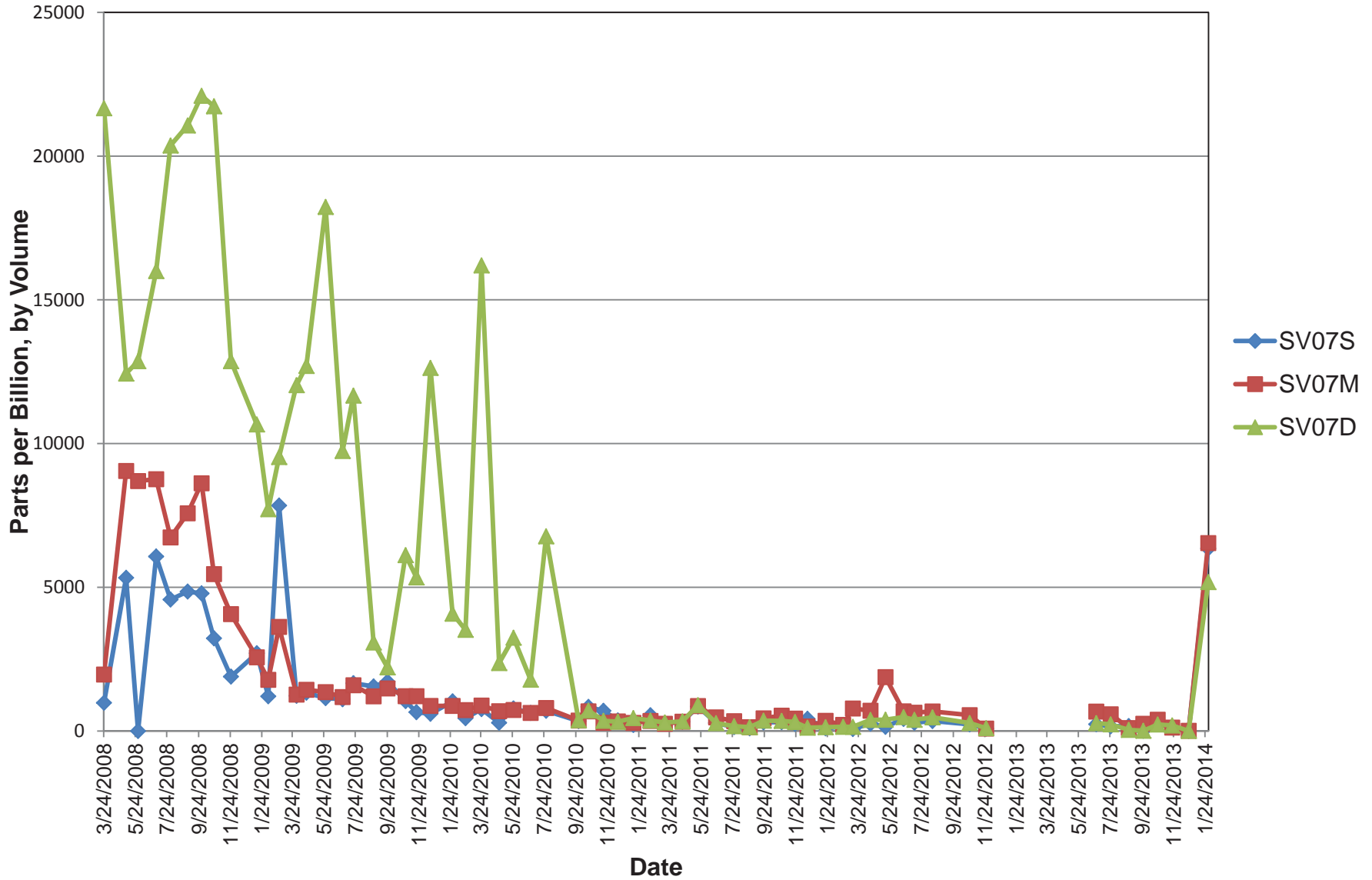
Figure 6 Soil Vapor Measurements SV07
