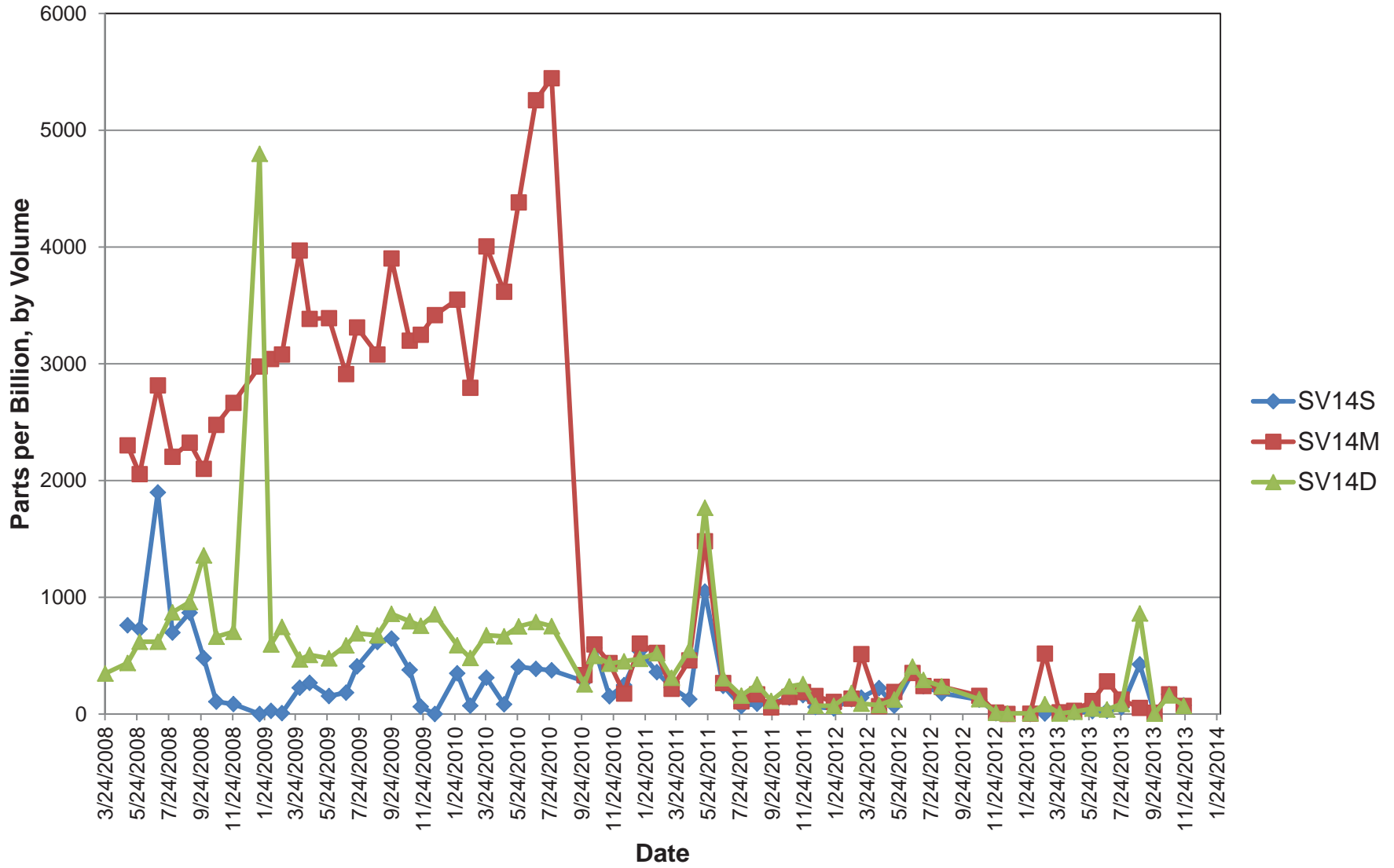
Figure 13 Soil Vapor Measurements SV14
