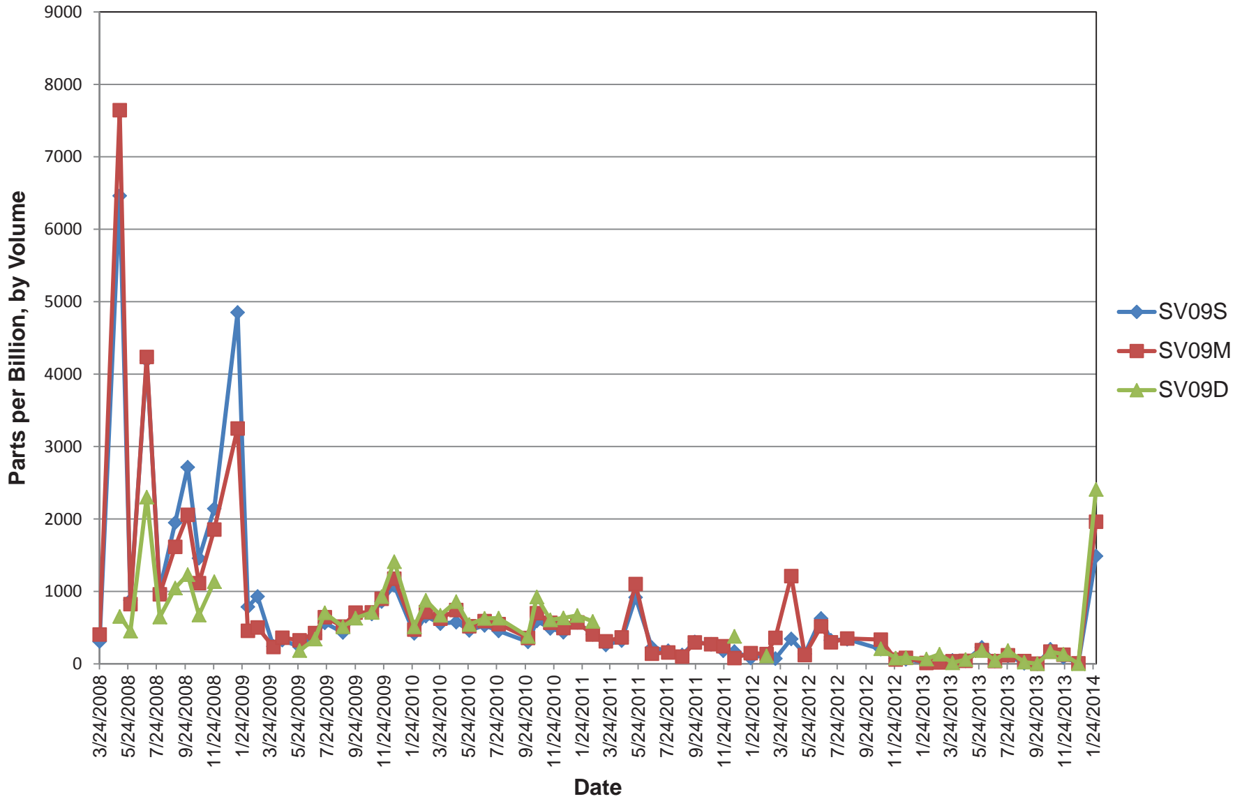
Figure 8 Soil Vapor Measurements SV09
