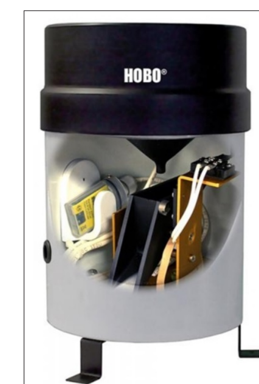
Gross Rainfall Equipment: Because the test plots are located close to one another, a single tipping bucket rain gauge (standard 8-inch diameter, 0.01-inch / tip) installed near the plots collects gross rainfall data to represent both the plots.
